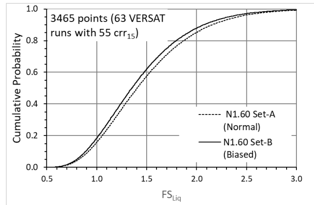
Fig. 10. Cumulative Probability Distribution Function (CDF) for FS_{Liq} (Element 12: 11.5 m depth)
